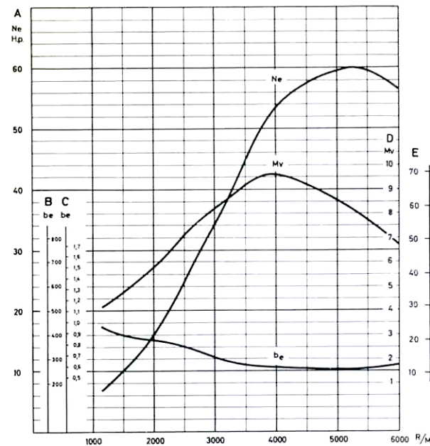
A=Power hp. B=g/hp. C=lb/hp. D=Torque kpm. E=Torque ft-lbs. Ne=Power, DIN. Mv=Torque. be=Fuel consumption per hph.
